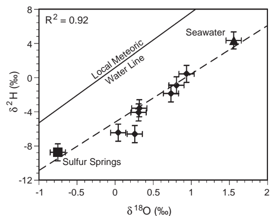
Fig. 5. Diagram showing \delta^{18}\text{O} and \delta^2\text{H} (both relative to VSMOW) of Champagne Hot Springs vent waters, Sulfur Springs, local precipitation and seawater. Data for the local meteoric water line from GNIP (IAEA/WMO, 2001).
